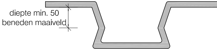
Detail taludgoot
